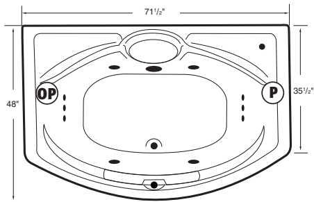
P Standard Pump Location OP Optional Pump Location
