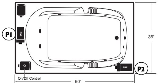
P1 Pump Location without skirt P2 Pump Location with skirt
