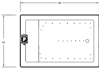
(P) Standard Pump Location
